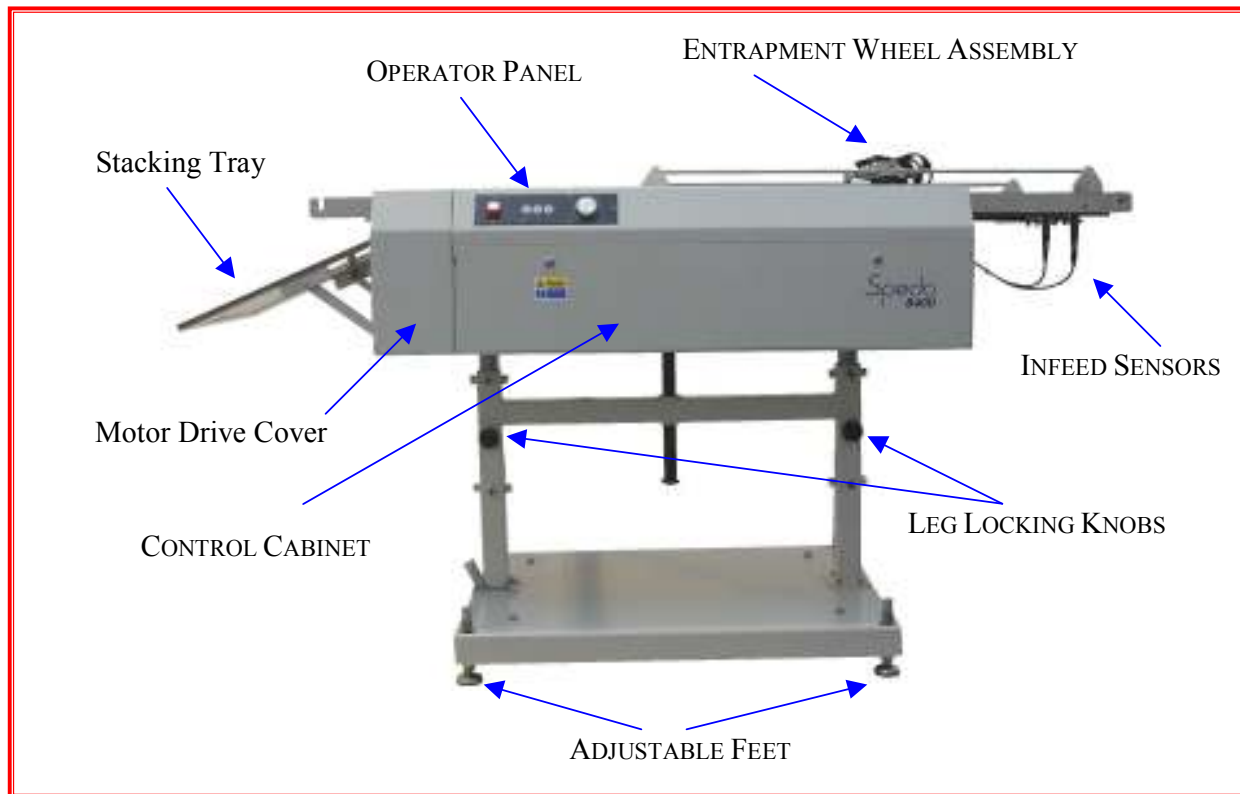
Fig 1.4 Identification of Main Assemblies
