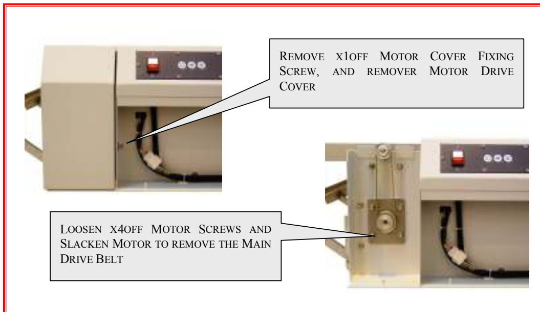
Fig 2.1 Replacing the Main Drive Belt
