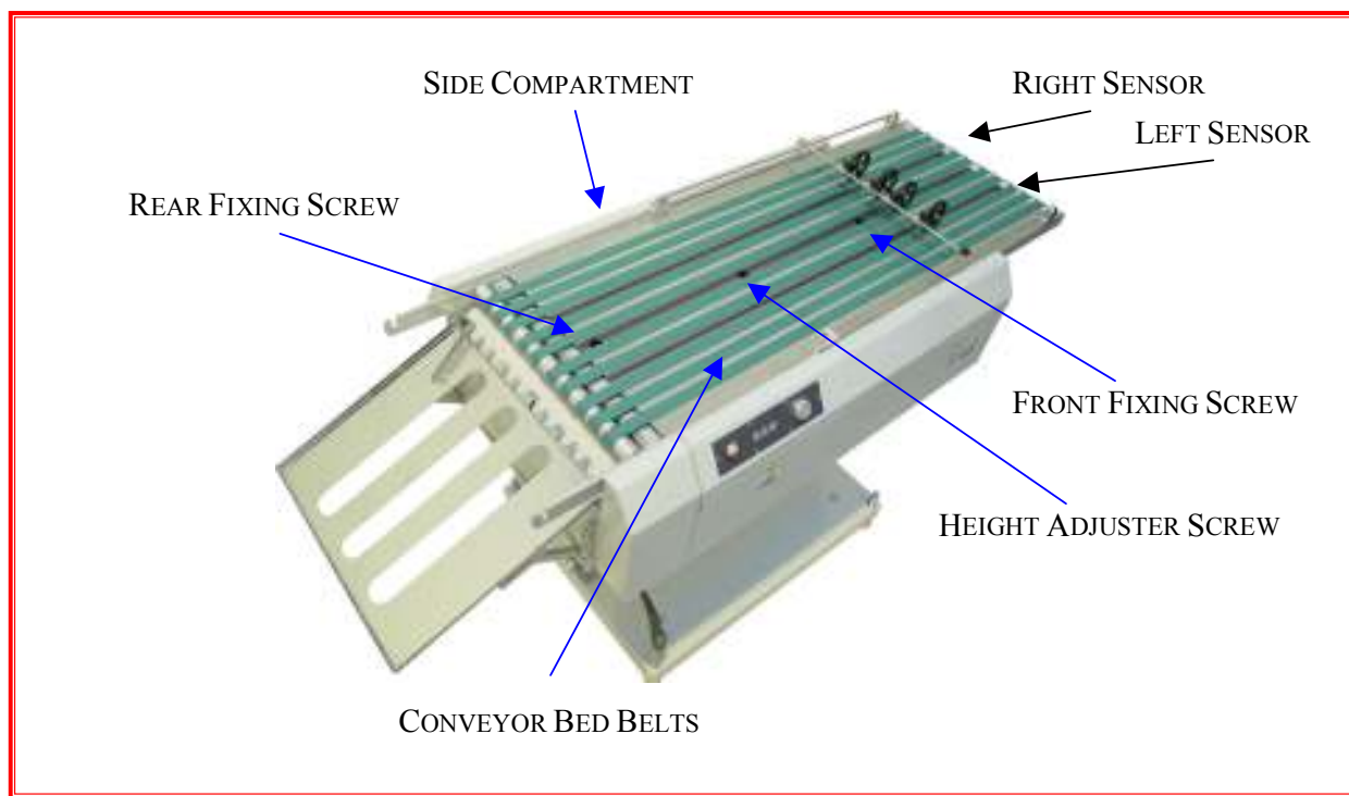
Fig 1.5 Identification of Main Assemblies
