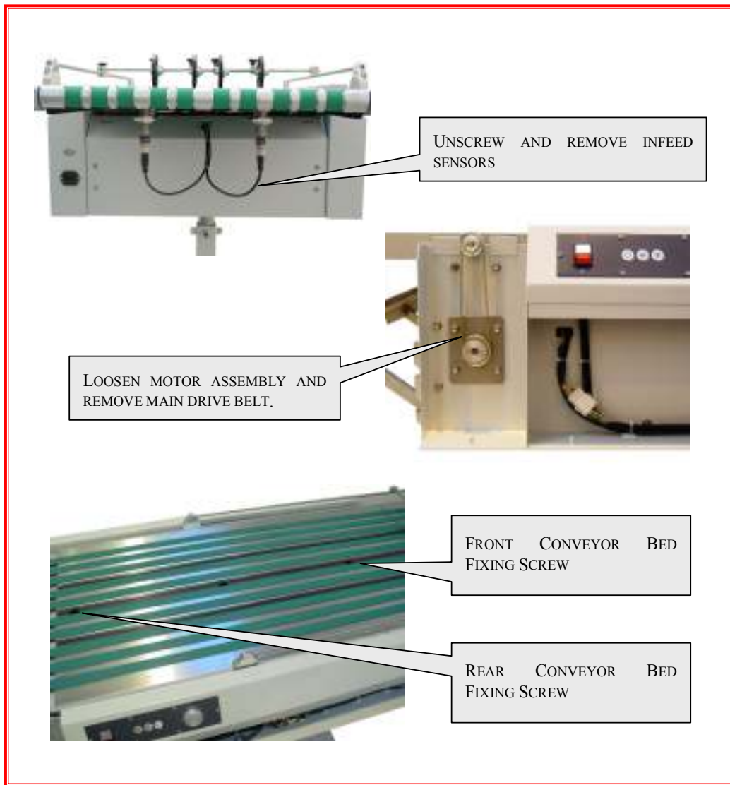
Fig 2.2 Replacement of Conveyor Bed Belts
